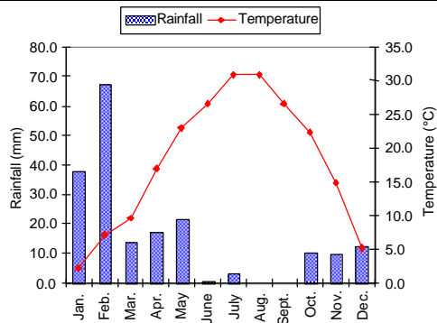
Fig. 1: Mean monthly rainfall and temperature (mean of 2007 &amp; 2008)
