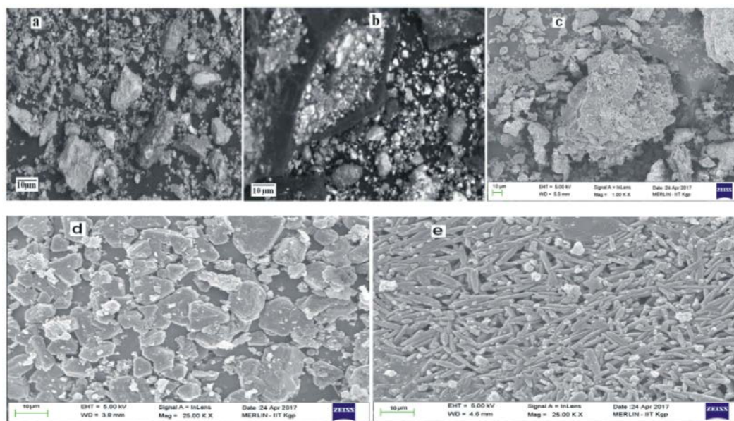
Fig. 2: SEM of granulated slag (a), air cooled slag (b), SMS slag (c), SMS sludge (d) and fly ash (e).
