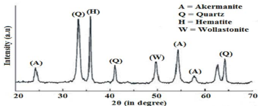
Fig. 4: XRD of Air cooled slag
