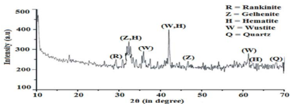
Fig. 3: XRD of granulated slag
