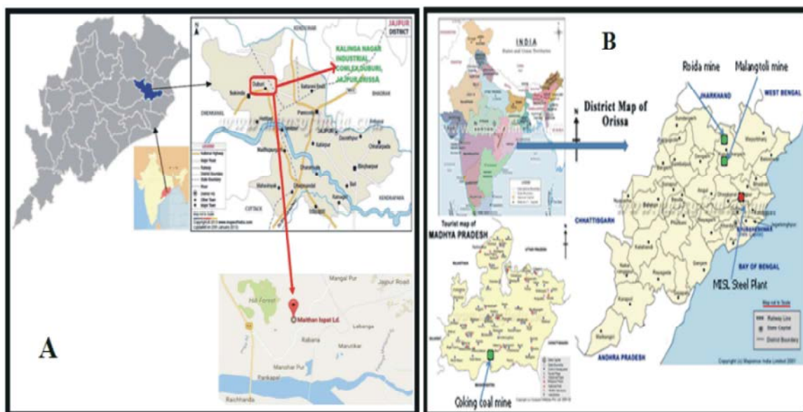
Fig. 1: Map showing the location of Kalinga Nagar Industrial Complex (KNIC) with Maithan Ispat Limited (A) and Mideast Integrated Steel Limited (MISL) – MESCO (B)
