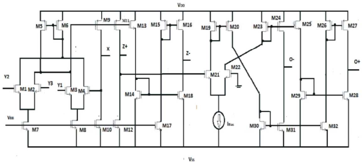
Fig. 2: The CMOS realization of modified DDCCTA [10]
