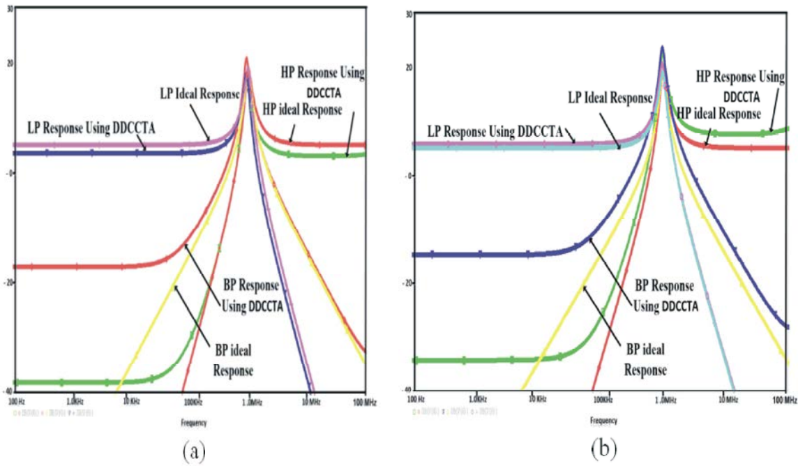
Fig. 9: (a) Magnitude Response of Fig. 8 (a) compare to ideal response (b) Magnitude Response of Fig. 8 (d) compare to ideal response
