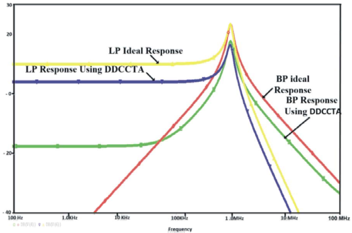
Fig. 13: Response of TT configuration of Fig. 12 (a) and ideal response
