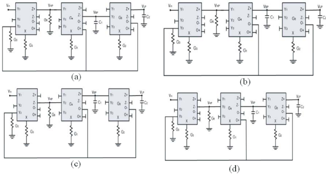
Fig. 8: (a) DDCCTA-KHN realizations type A (a) Class I (b) Class II (c) Class III (d) Class IV
