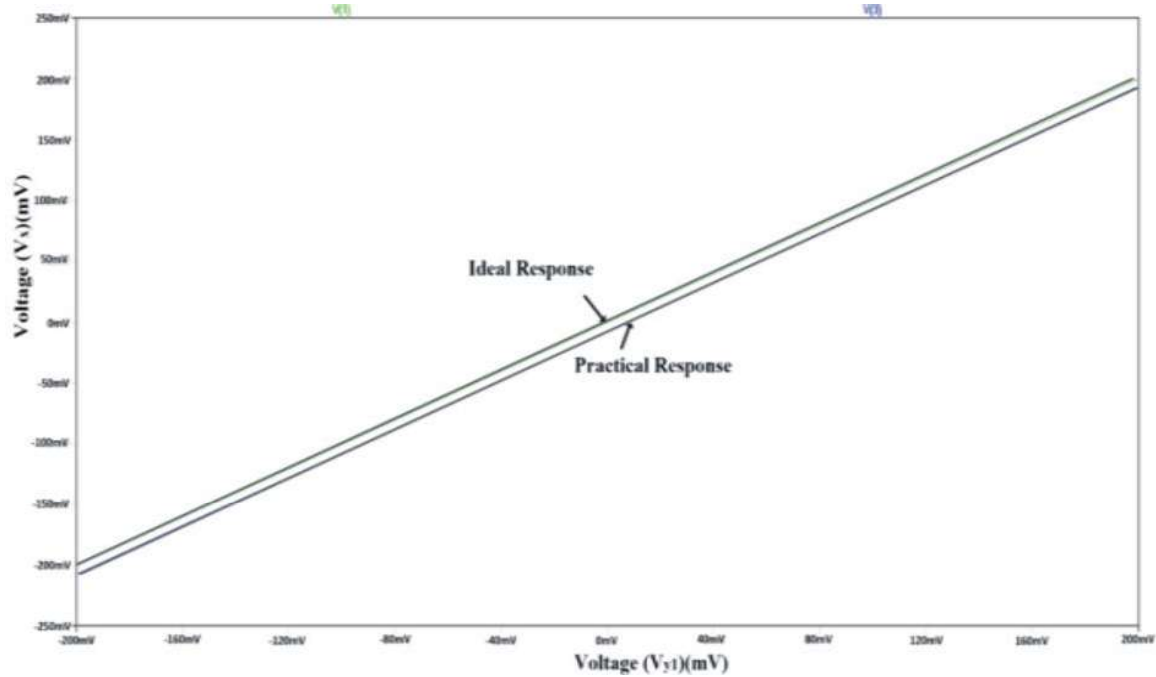
Fig. 4: DC transfer characteristic for voltage transfer from Y1 port to X port
