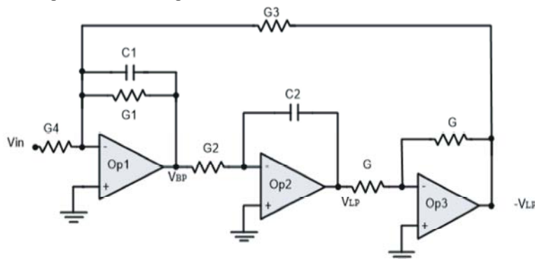
Fig. 11: Tow-Thomas (TT) second order filter using three Op Amps [25, 26]
