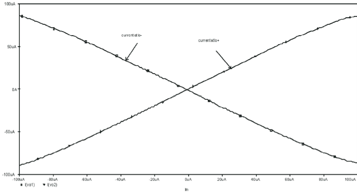
Fig. 6: DC transfer characteristic for current transfer from X port to O+ and O-
