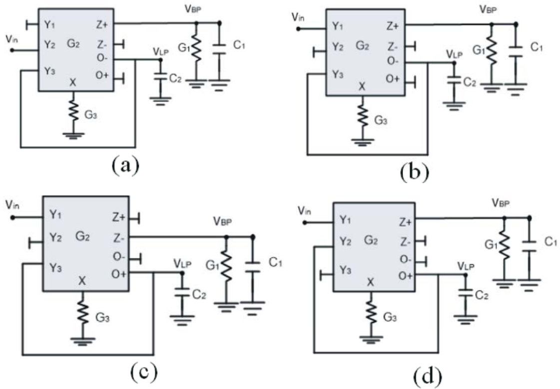
Fig. 12: DDCCTA-TT Realizations(a) Class A (b) Class B (c) Class C (d) Class D
