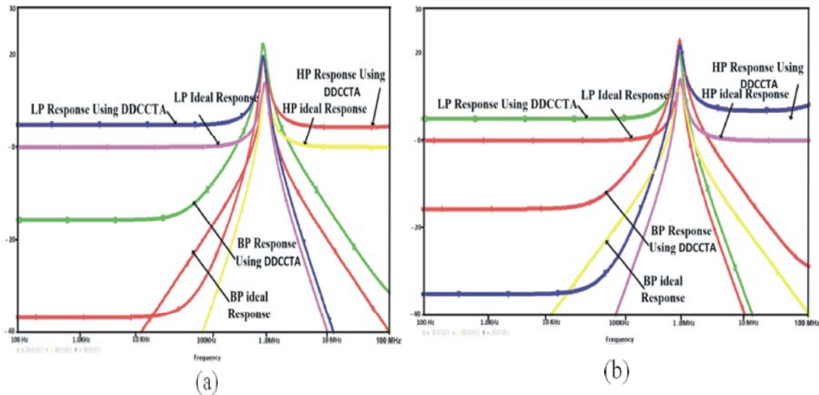
Fig. 10: (a) Magnitude Response of KHN type B class I compared to ideal response (b) Magnitude Response of KHN type B class IV compared to ideal response
