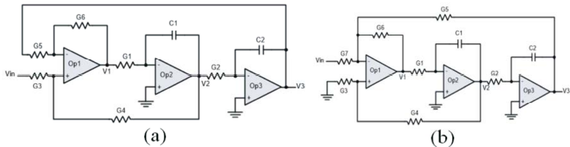
Fig. 7: (a) Type A KHN circuit using three op amps [2]. (b) Type B inverted KHN circuit using three op amps [50]
