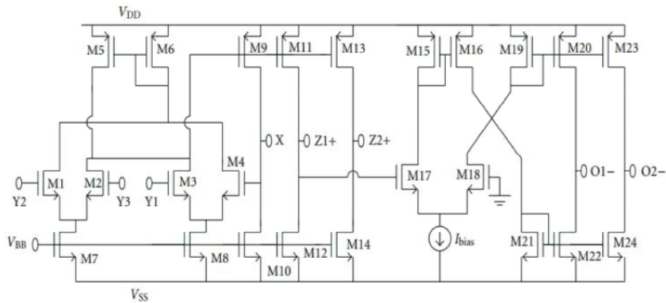
Fig. 1: The CMOS realization of the DDCCTA[10]
