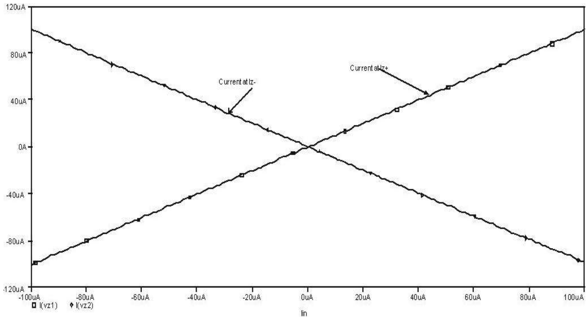
Fig. 5: DC transfer characteristic for current transfer from X port to Z+ and Z- Ports.
