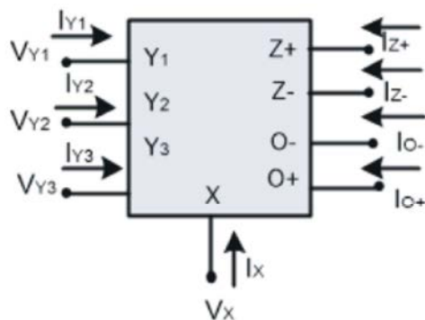
Fig. 3: Circuit symbol of the DDCCTA
