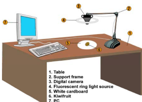
Fig. 1: Image acquisition system
