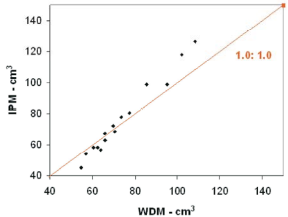
Fig. 5: Kiwifruit volume measured using water displacement method (WDM) and image processing method (IPM) with the line of equality (1.0: 1.0)
