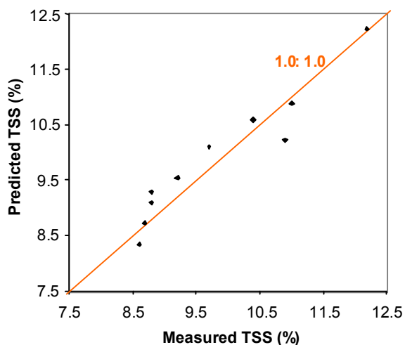
Fig. 1: Measured TSS and predicted TSS with the line of equality (1.0: 1.0)
