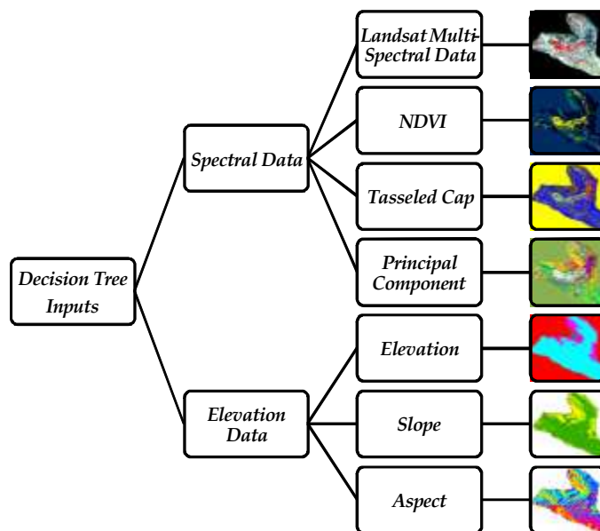
Fig. 4: Decision tree inputs including spectral and elevation data
