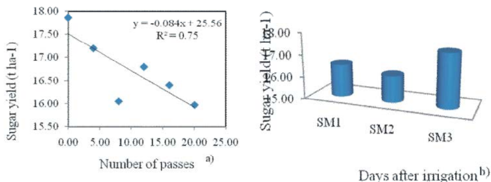
Fig. 6: Sugar cane yields as affected by number of tractor passes (a) and soil moisture levels (b)
