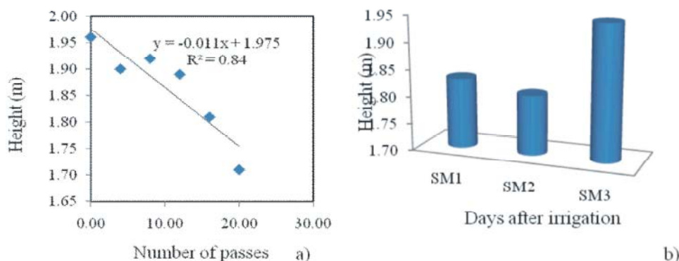
Fig. 5: Sugarcane height as affected by number of tractor passes (a) and soil moisture levels (b)
