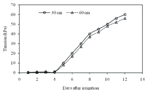
Fig. 3: Soil moisture calibration curve for the study site
