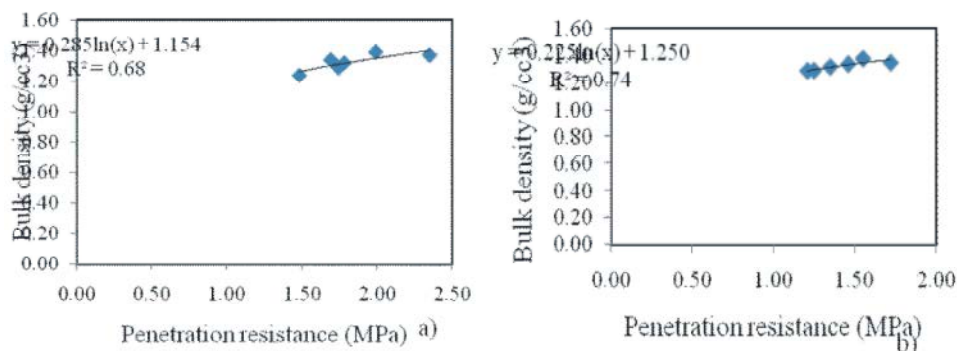
Fig. 4: Relationship between bulk density and soil penetration resistance in response to soil compaction (a) for topsoil layer and (b) for subsoil layer
