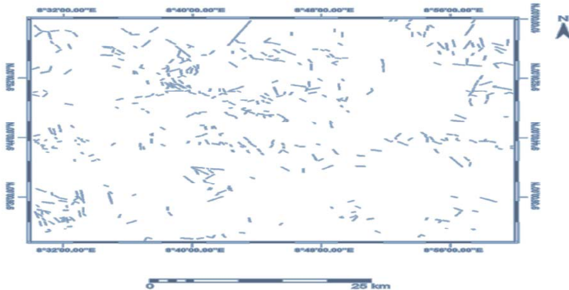
Fig. 3: Map of Lineaments Extracted from Spot Image of the Study Area
