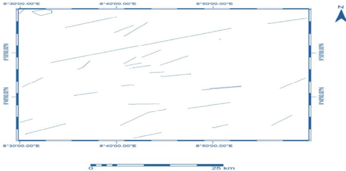
Fig. 2: Map of Lineaments Extracted from Aeromagnetic map of the study area
