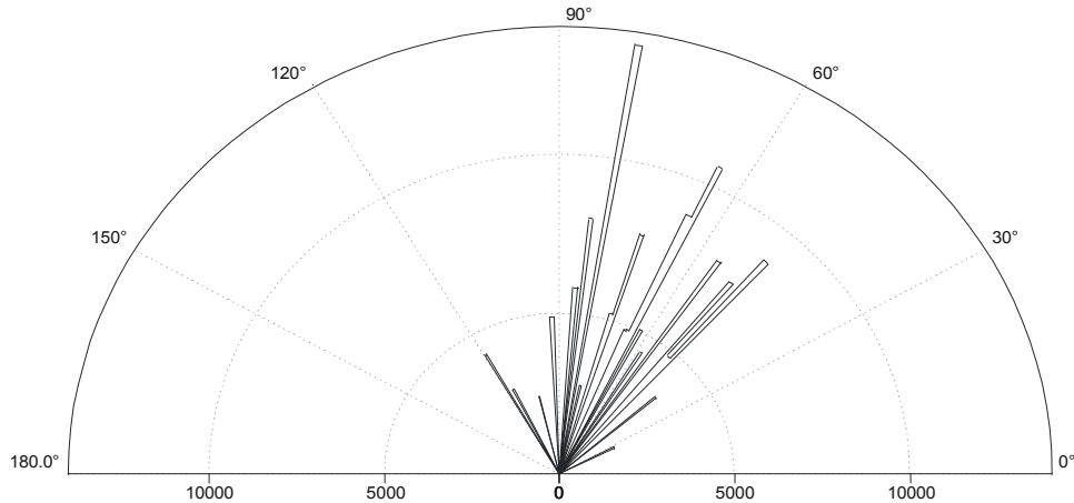
Fig. 9: Rose Plot of Lineaments derived from Aeromagnetic Data of the Study Area
