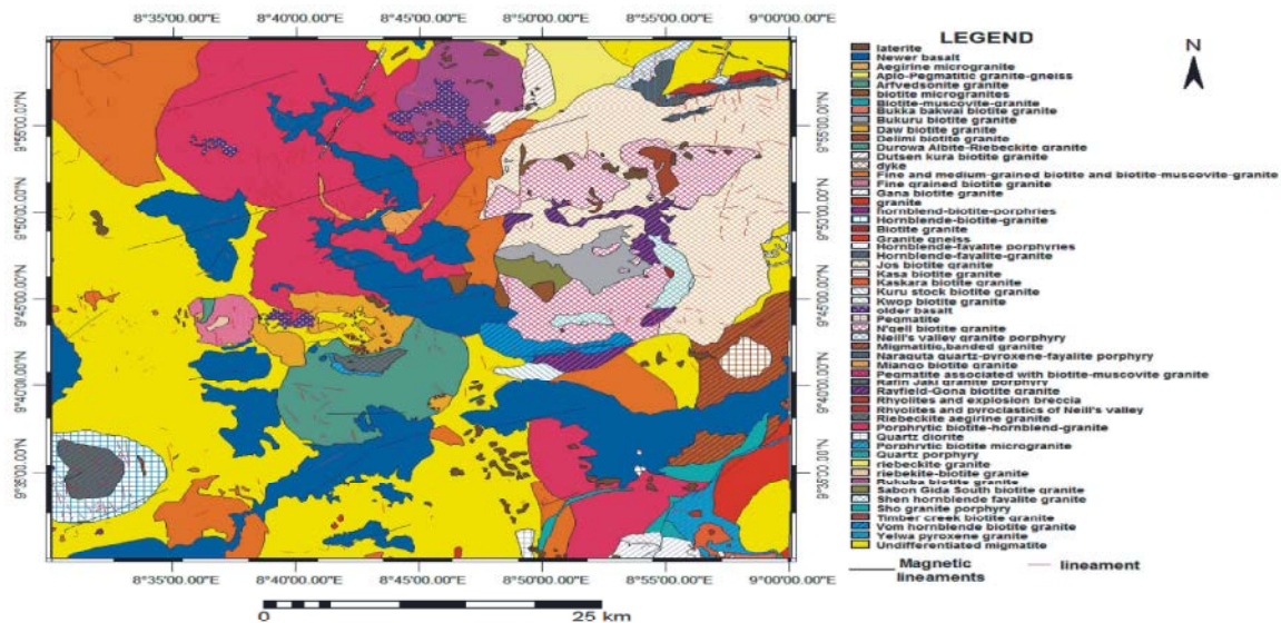
Fig. 1: Geological Map of Study Area overlain with Magnetic Lineaments and Lineaments Extracted from Spot Image. (Modified GSN)
