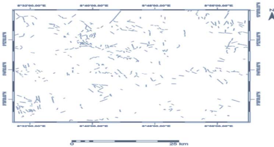
Fig. 6b: Map of Lineaments Extracted from Spot Image of the Study Area
