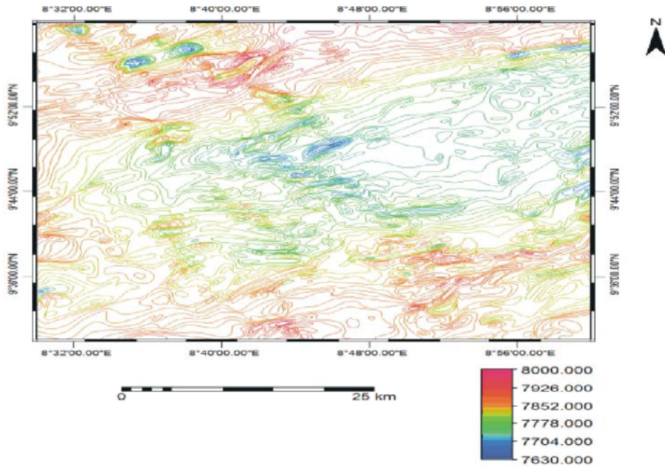
Fig. 2: Digitized Aeromagnetic Map of Study
