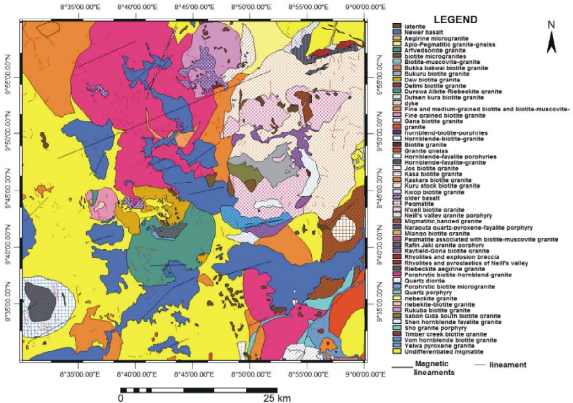
Fig. 7: Geological Map of Study Area overlain with Magnetic Lineaments and Lineaments Extracted from Spot Image. (Modified GSN)
