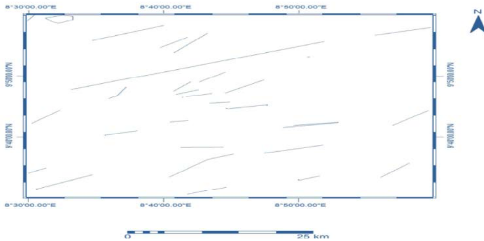
Fig. 6a: Map of Lineaments Extracted from Aeromagnetic map of the study area
