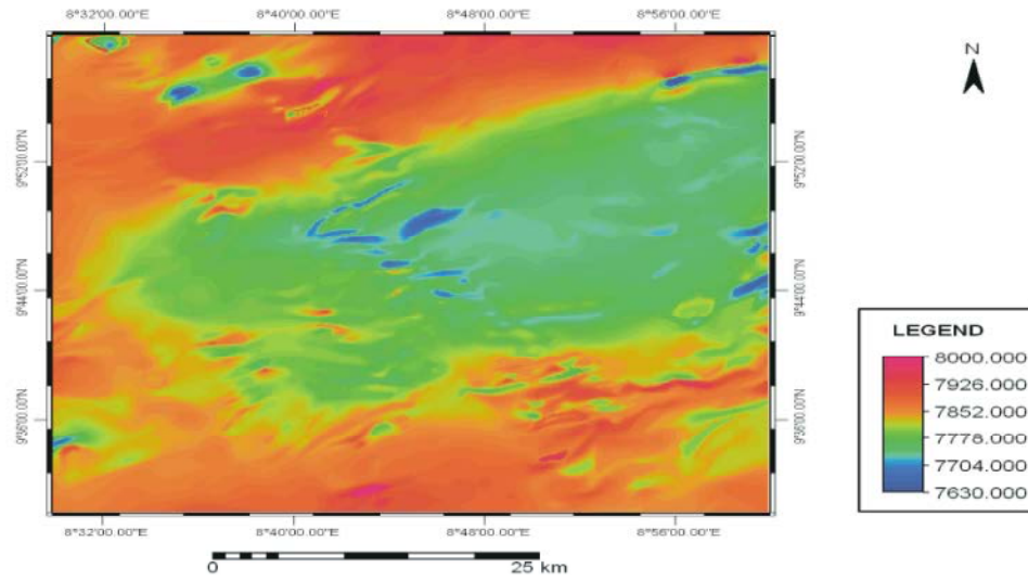
Fig. 5: Interpolated Aeromagnetic Map of the Study Area
