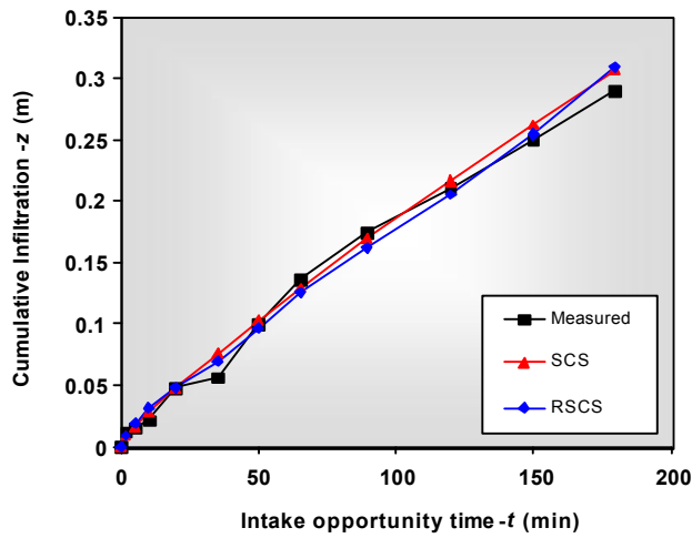
Fig. 2: Cumulative infiltration predicted using SCS and RSCS models compared with that measured experimentally for treatment 1
