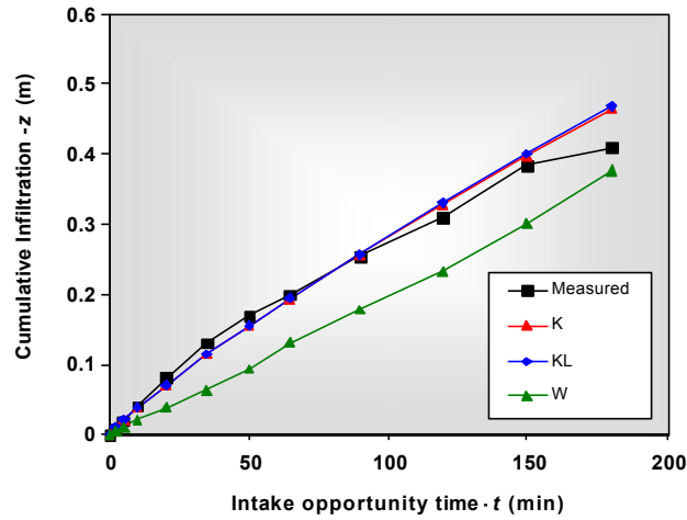
Fig. 3: Cumulative infiltration predicted using K, KL and W models compared with that measured experimentally for treatment 2
