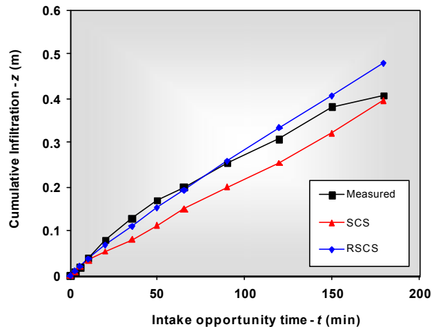
Fig. 4: Cumulative infiltration predicted using SCS and RSCS models compared with that measured experimentally for treatment 2
