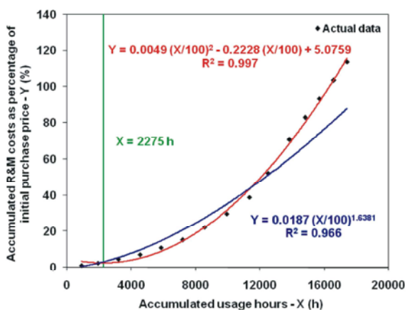
Fig. 2: Curves of predicted accumulated R&M costs as percentage of initial purchase price based on accumulated usage hours using the power and polynomial regression models for MF-285 tractors under study
