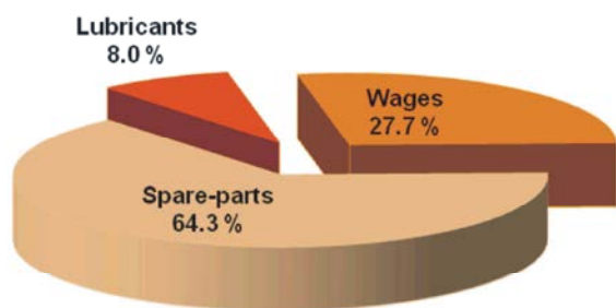
Fig. 1: Mean R&M costs fractions, i.e. spare-parts, wages and lubricants for U-650 tractors under study
