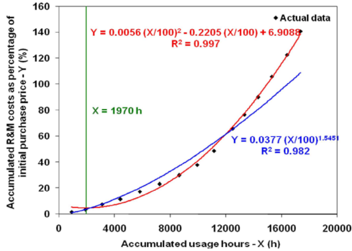
Fig. 2: Curves of predicted accumulated R&M costs as percentage of initial purchase price based on accumulated usage hours using the power and polynomial regression models for U-650 tractors under study
