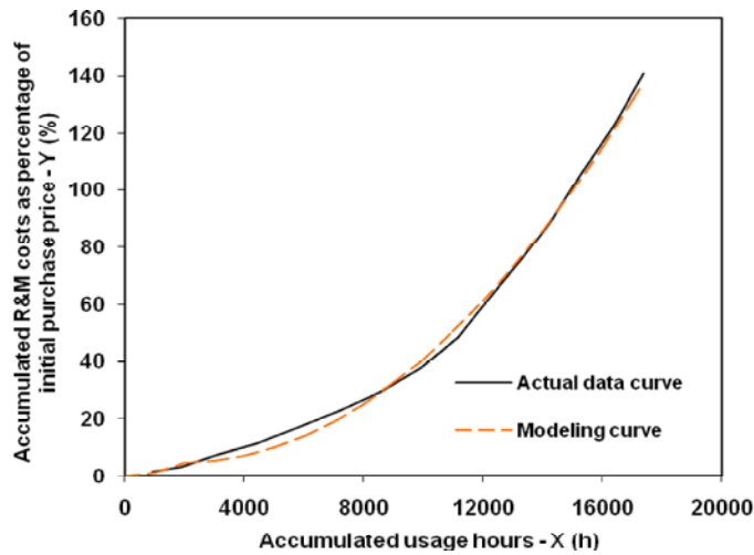
Fig. 3: Actual data curve and modeling curve of accumulated R&M costs based on accumulated usage hours for U-650 tractors under study
