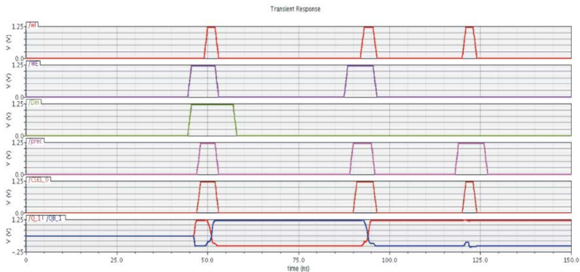
Fig. 6: Simulation waveform of SRAM cell write operation
