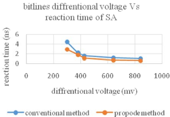
Fig. 10: Comparison graph of the convention and proposed SA read operation
