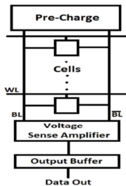
Fig. 1: Column circuit of SRAM Array
