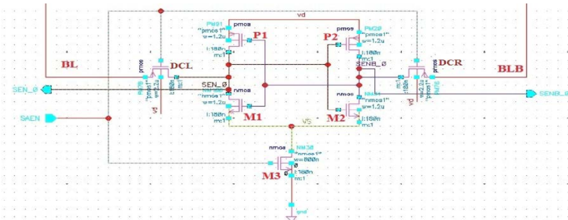
Fig. 4: Conventional Sense Amplifier Circuit
