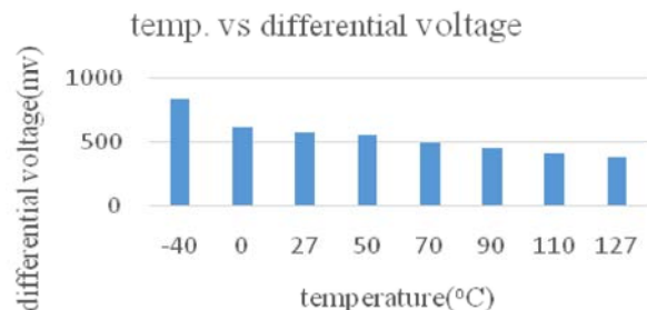
Fig. 8: Temperature impact on bit line differential voltage
