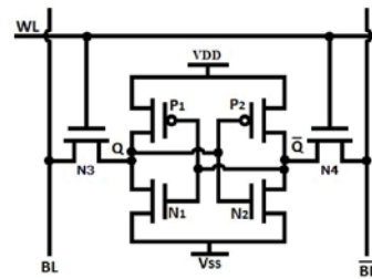
Fig. 2: 6T SRAM cell
