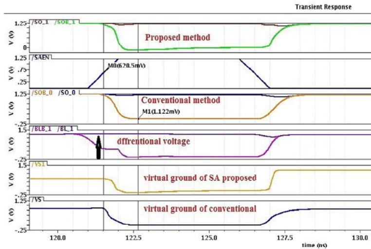
Fig. 7: The simulation waveform for proposed and conventional sense amplifier read operation
