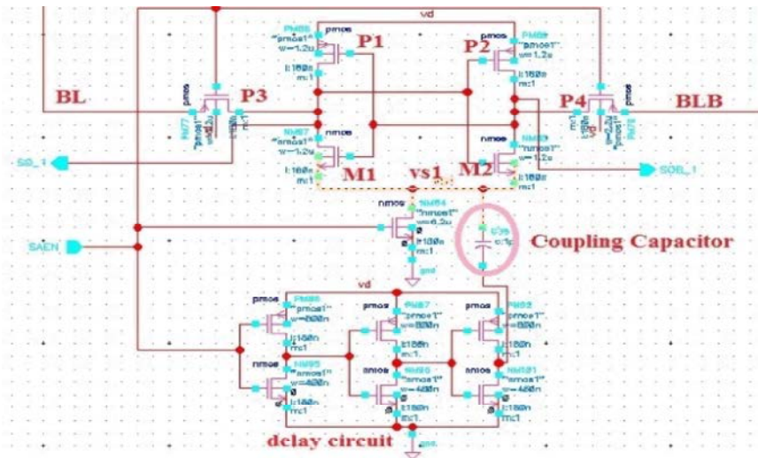
Fig. 5: Coupling capacitor based sense amplifier
