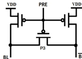
Fig. 3: Bit line precharge circuit
