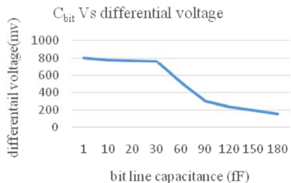
Fig. 9: Impact of bit line capacitance on generation of differential voltage
