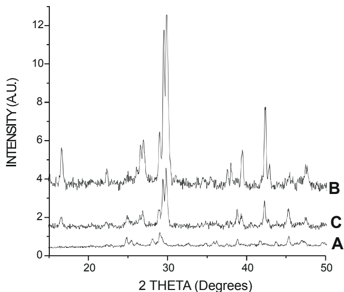
Fig. 1: XRD Patterns of the sol-gel-synthesized samples A, B and C
