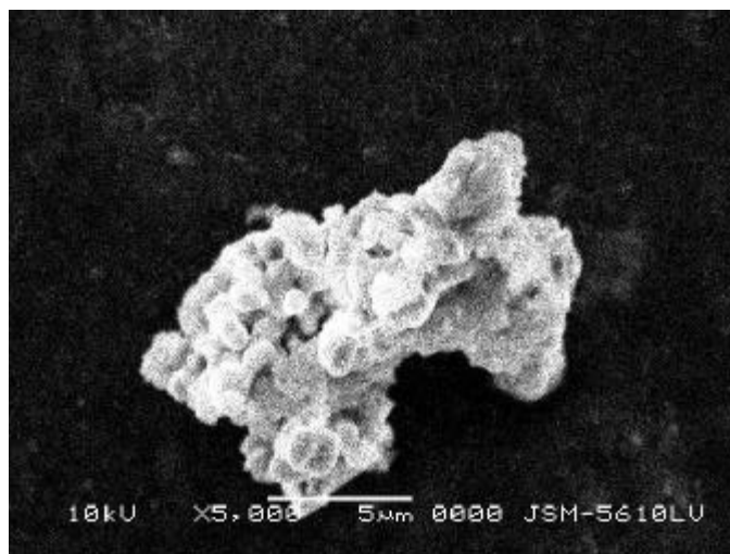
Fig. 2: SEM of sol-gel synthesized sample at 1200°C
