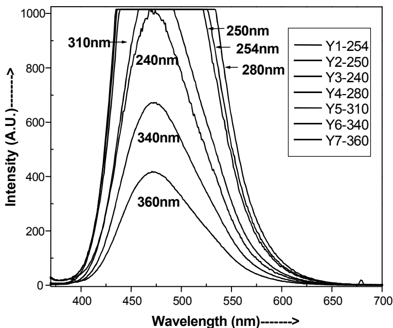
Fig. 4: The photoluminescence emission spectra of the sol-gel synthesized sample at different excitation wavelengths.
