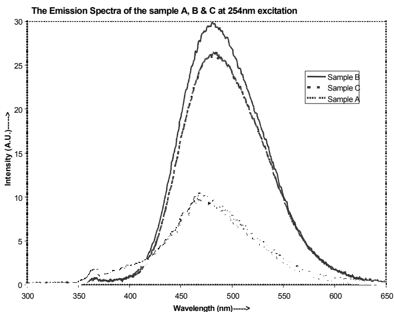
Fig. 3: The photoluminescence emission spectra of the \text{Sr}_2\text{CeO}_4 sol-gel synthesized sample excited at 254nm
