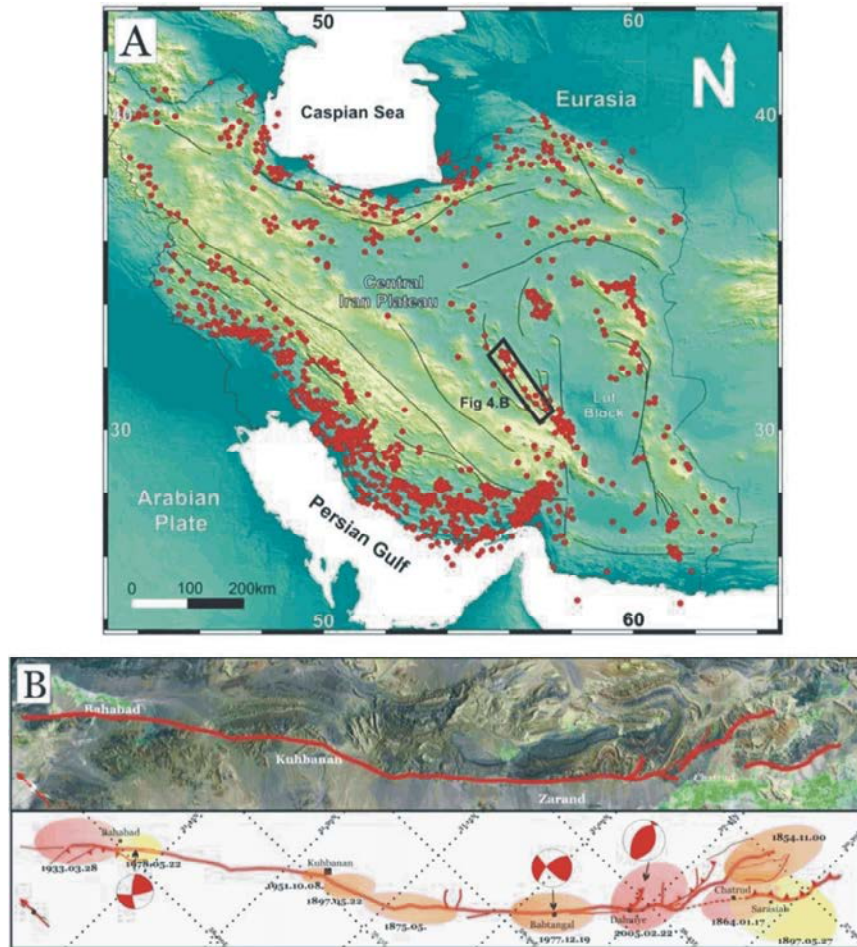
Fig. 4: A) Seismicity of Iran with epicenters from the catalogue of Engdhal et al. (2005). B) Meisoseismal of areas around of Kuhbanan fault system
