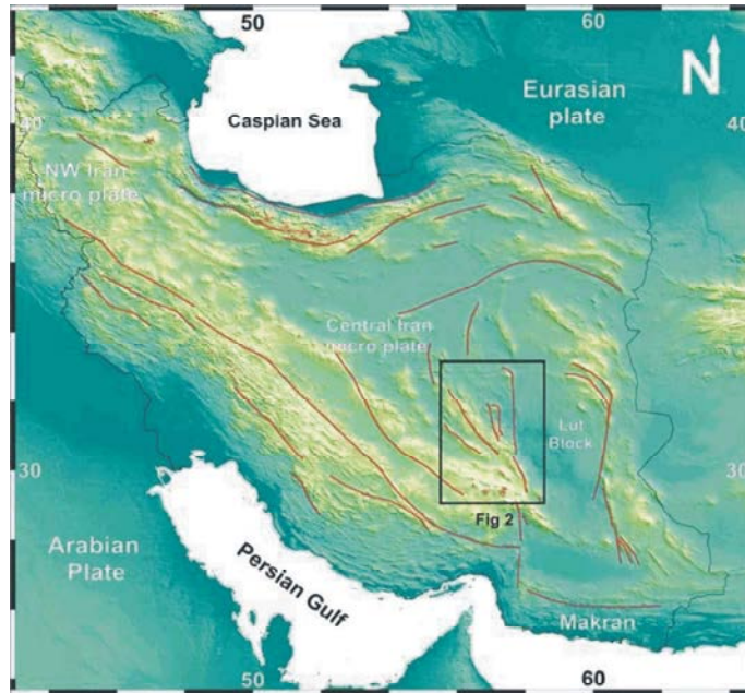
Fig. 1: Main structural unites of Iran and surrounds Plates.
