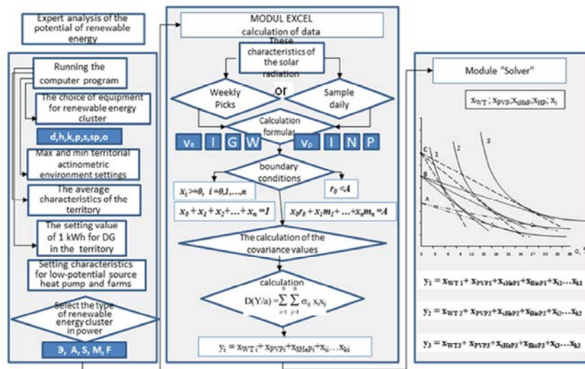
Fig. 3: Algorithm for computation of the optimal RES cluster based on the stochastic data of long-term observations of actinometric characteristics
