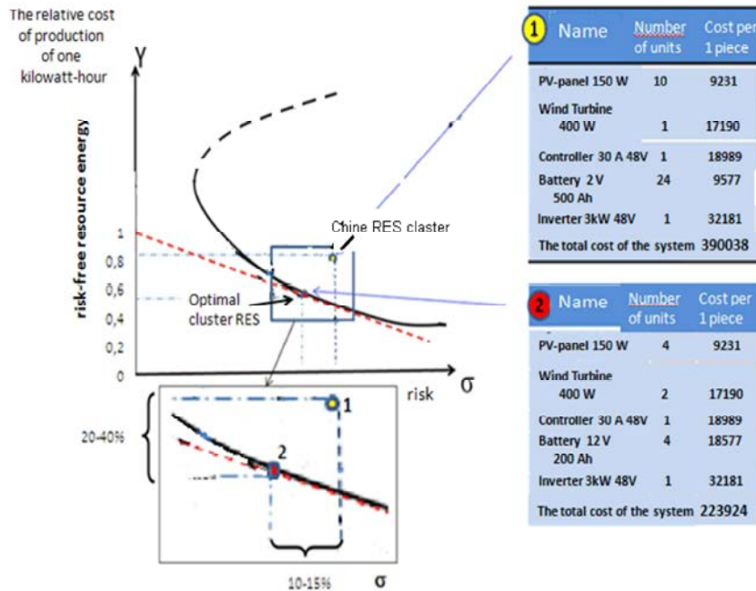
Fig. 5: Graphical comparison of the regular model kit d-cluster RES China (1) and the renewable energy cluster (2) of the same manufacturer optimized by the program "ARC-RES"
