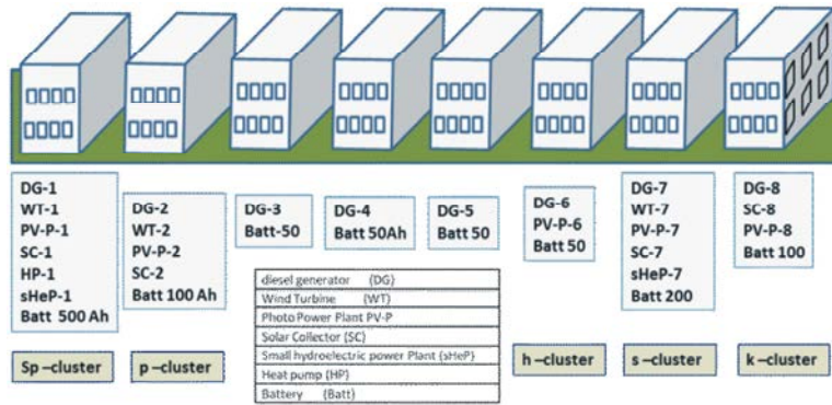
Fig. 2: Composition of the equipment of the RES clusters in the apartments of the “Energy Efficient House”
