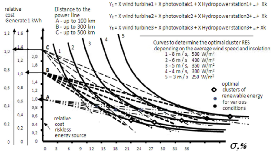
Fig. 6: Diagram for comparing the optimal RES clusters depending on the relative cost of generation of 1 kWh as a function of distance to the central energy sources (power lines) and actinometric parameters at the consumer's site.
