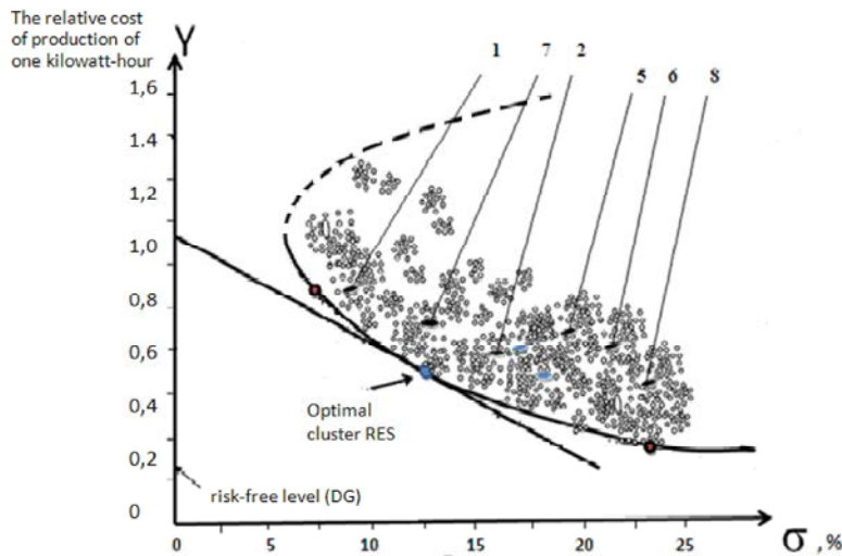
Fig. 4: The experimental data for apartments (1-8) corresponding to clusters of RES and the design characteristics of the optimal cluster RES.
