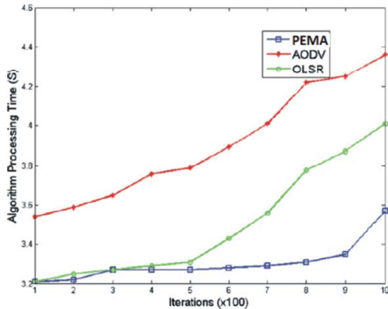
Fig. 3: Comparative Analysis of PEMA, AODV and OLSR (Algorithm Processing Time)
