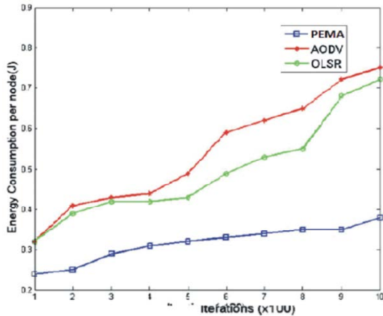
Fig. 2: Comparative analysis of PEMA, AODV, OLSR (Power)
