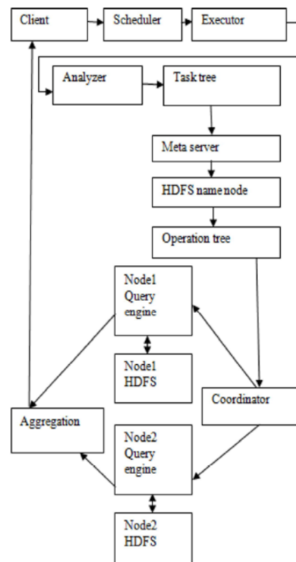
Fig. 4: Workflow of splitting and scheduling
