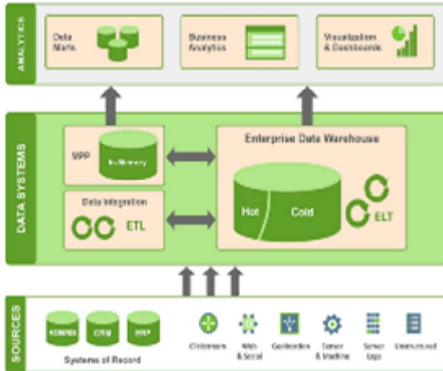
Fig. 1: Cloud Environment
