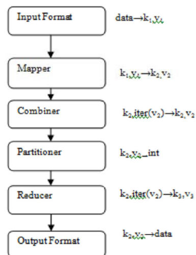
Fig. 2: Map Reduce steps
