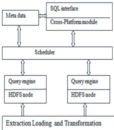
Fig. 3: Banian Architecture
