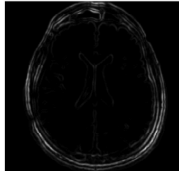
Fig. 5.h: Indeterminate image
