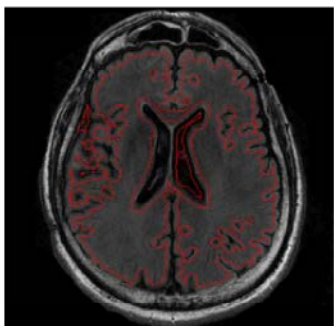
Fig. 5.j: Segmented area
