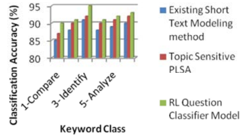
Fig. 5: Measure of Classification Accuracy
