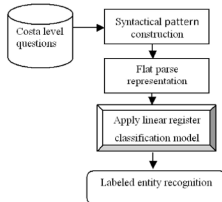
Fig. 1: Architecture Diagram of Register Linear (RL) Classification Model
