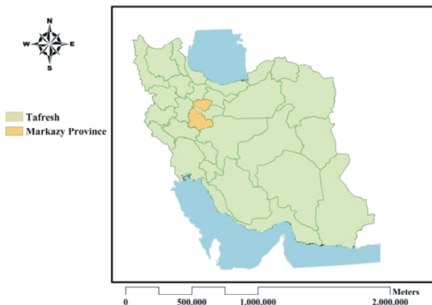
Fig. 1: Markazi Province in Iran
