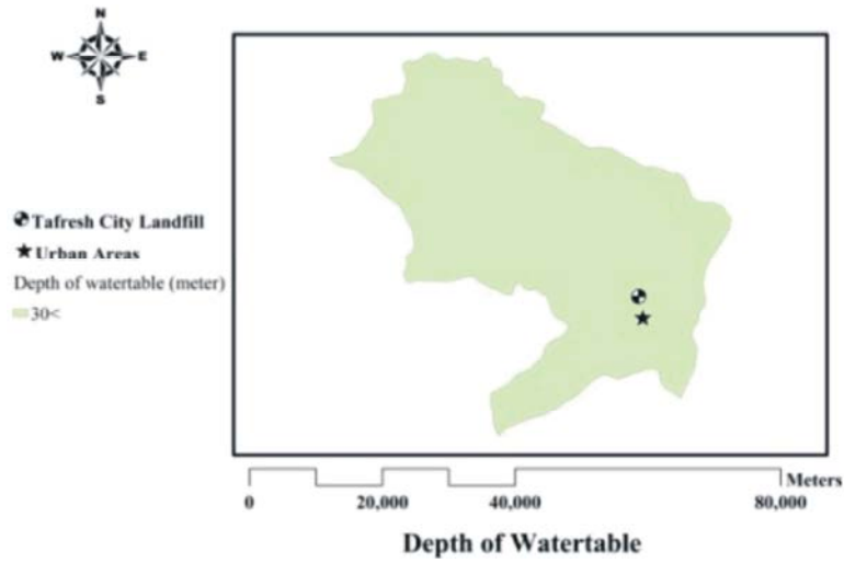
Fig. 6: Areas Even with Groundwater in Depth
