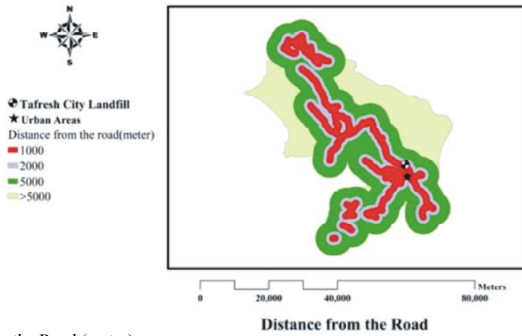
Fig. 3: Distance from the Road (meter)
