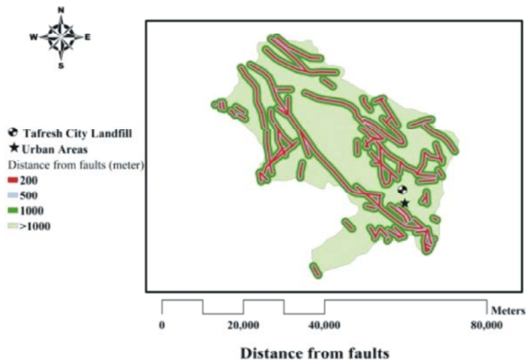
Fig. 5: Distance from Faults (meter)
