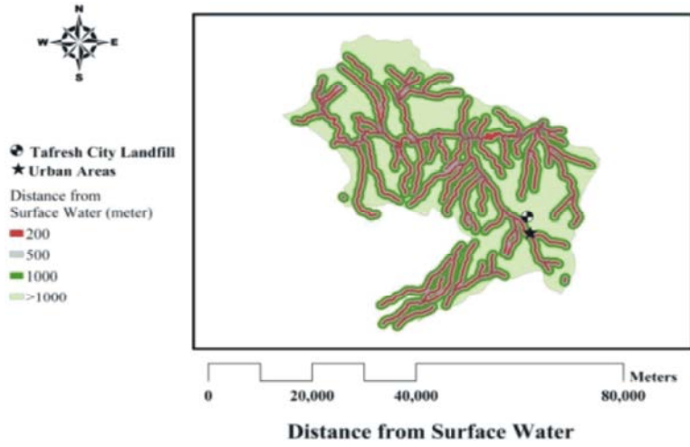
Fig. 7: Distance from River (meter)
