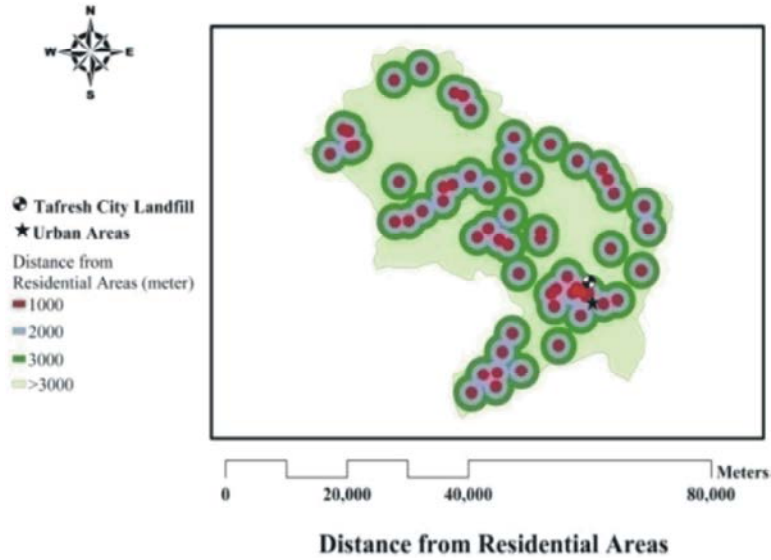
Fig. 10: Distance from Residential Areas
