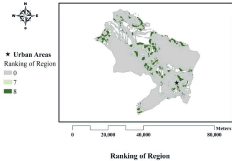
Fig. 15: Ranking of Regions Based on Final Score
