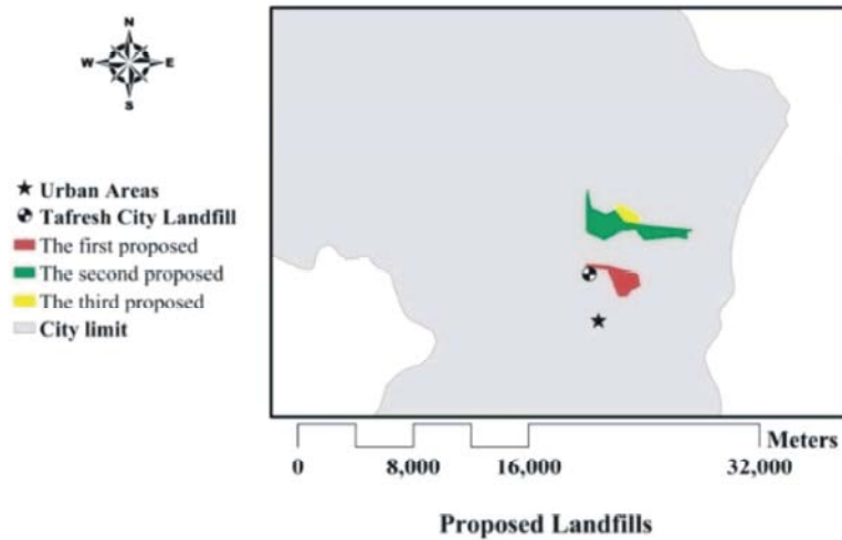
Fig. 16: Proposed landfill sites for the city Tafresh
