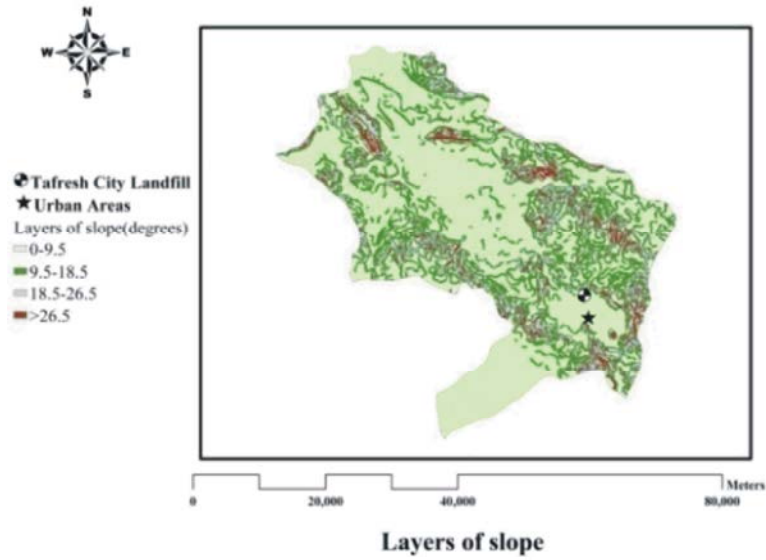
Fig. 4: Regional Classified Slope
