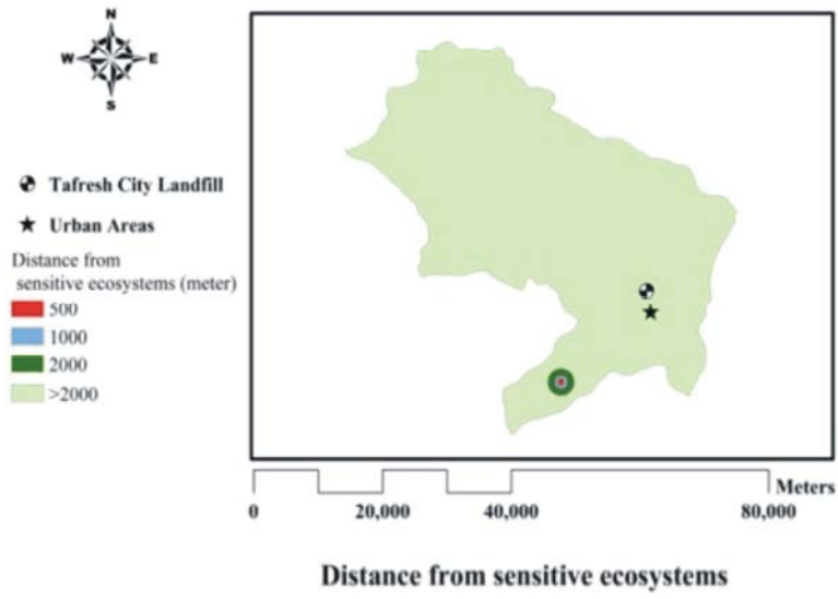
Fig. 9: Distance from Sensitive Ecosystems
