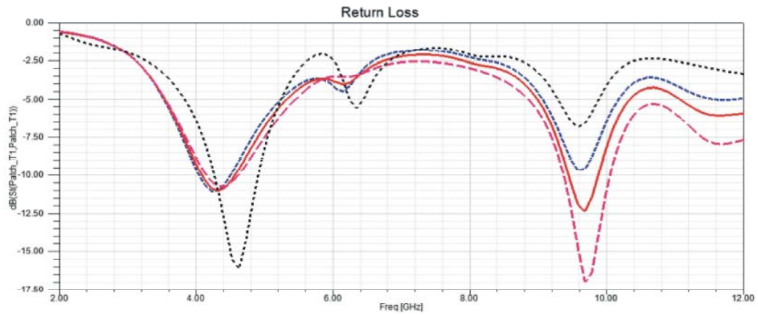
Fig. 6: Parametric analysis for change in d_4
