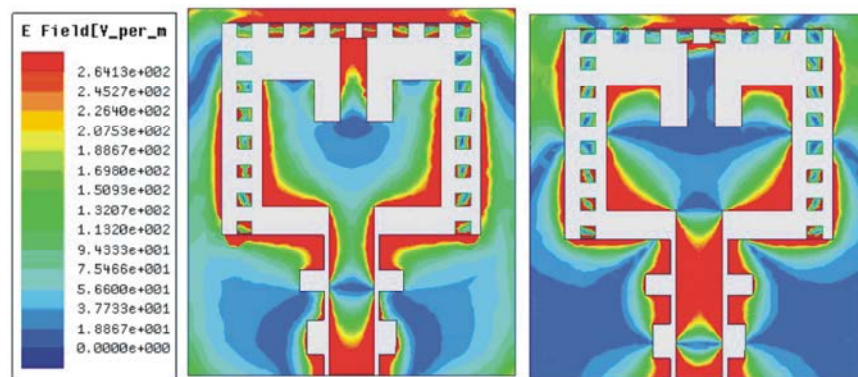
Fig. 10: E-Field Distribution on the antenna with EBG at 4.4 and 9.6 GHz
