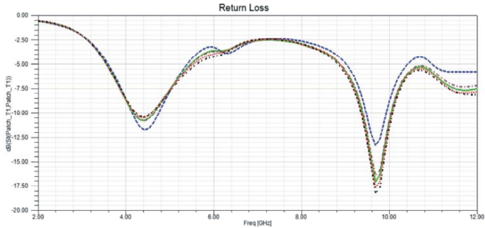
Fig. 4: Parametric analysis for change in b1
