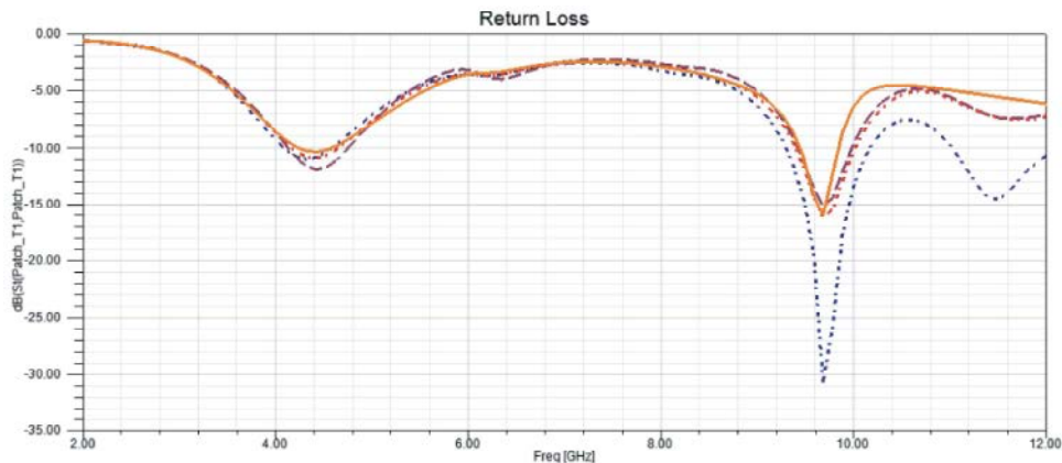
Fig. 5: Parametric analysis for change in d2
