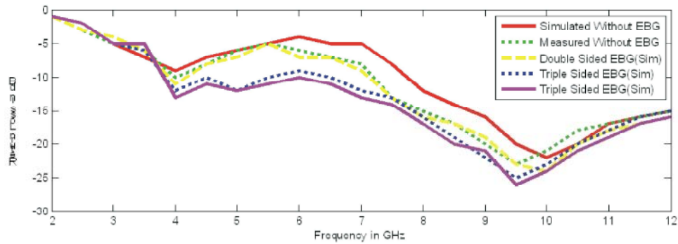
Fig. 3: Measured and Simulated Return loss Vs Frequency curve
