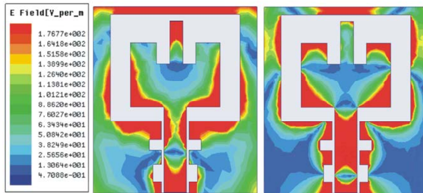
Fig. 9: E-Field Distribution on the antenna without EBG at 4.4 and 9.6 GHz
