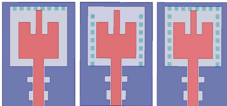
Fig. 2(a): Single Sided EBG, Fig. 2(b): Double Sided EBG, Fig. 2(c): Triple Sided EBG
