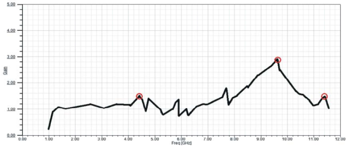
Fig. 8: Frequency Vs Gain
