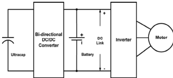
Fig. 2: UC/battery configuration
