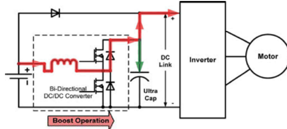
Fig. 12: Phase 2 Acceleration
