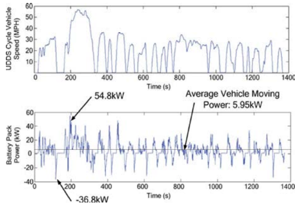
Fig. 7: Simulation results
