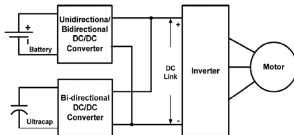
Fig. 5: Multiple converter configuration.
