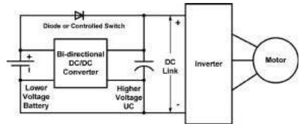
Fig. 8: Proposed HESS configuration
