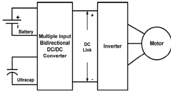
Fig. 6: Multiple input converter configuration
