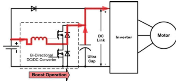
Fig. 11: Phase 1 Acceleration
