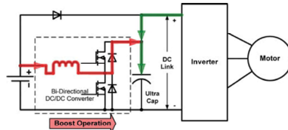
Fig. 13: Deceleration
