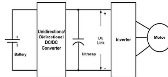
Fig. 3: Battery/UC configuration
