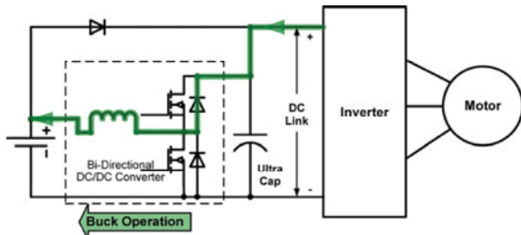
Fig. 15: Deceleration phase II
