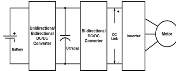
Fig. 4: Cascaded configuration
