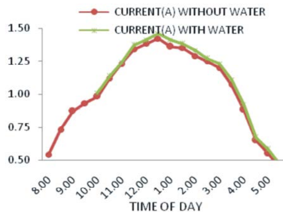
Fig. 6: Comparison of current with and without spraying water
