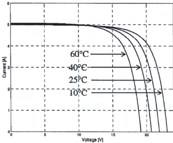
Fig. 1: I-V Characteristics at different temperature
