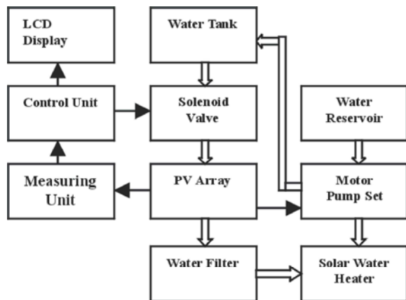
Fig. 2: Layout of PVPS with spraying Unit
