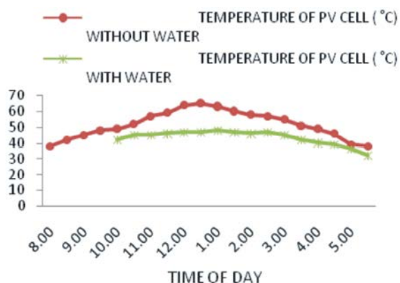
Fig. 7: Comparison of cells temperature with and without spraying water
