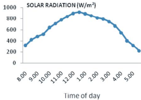
Fig. 4: Variation of Solar radiation
