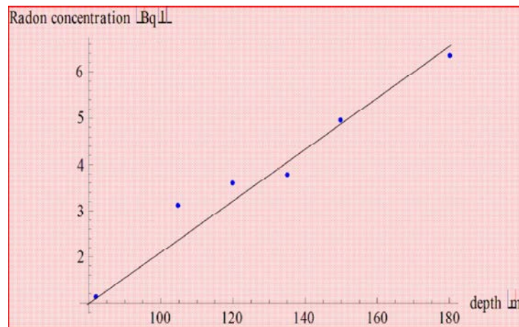
Fig. 7: The amount of Radon concentration in samples to the wells depth and the best fit
