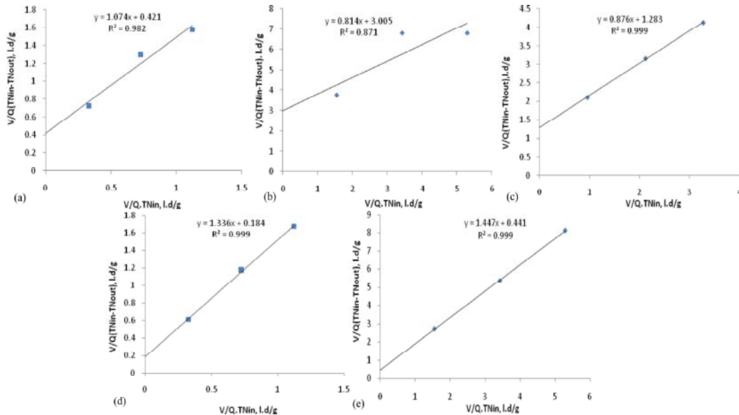
Fig. 6: Stover-Kincannon model plots for TN removal in, (a) aeration time = 30 min/h and COD/N ratio = 4, (b) aeration time = 30 min/h and COD/N ratio = 20, (c) aeration time = 40 min/h and COD/N = 12, (d) aeration time = 50 min/h and COD/N ratio = 4, (e) aeration time = 50 min/h and COD/N ratio = 4.
