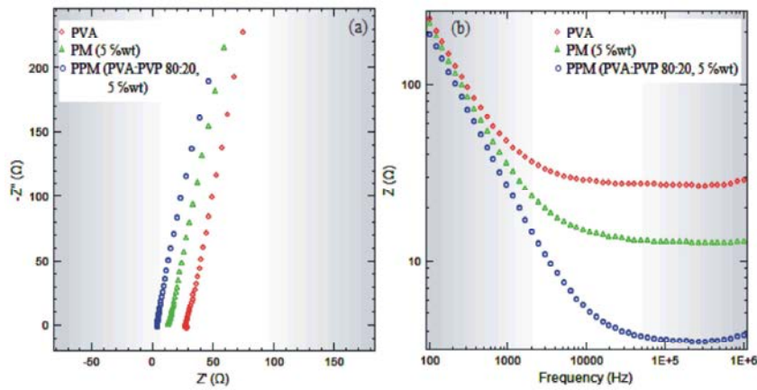
Fig 2: Nyquist (a) and bod (b) plots of PVA and nanocomposite membranes
