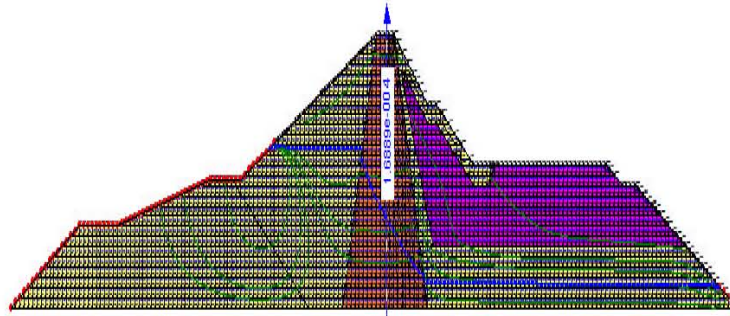
Fig. 4: Flow rate under earth dams at elevation of (120 m) above the free surface
