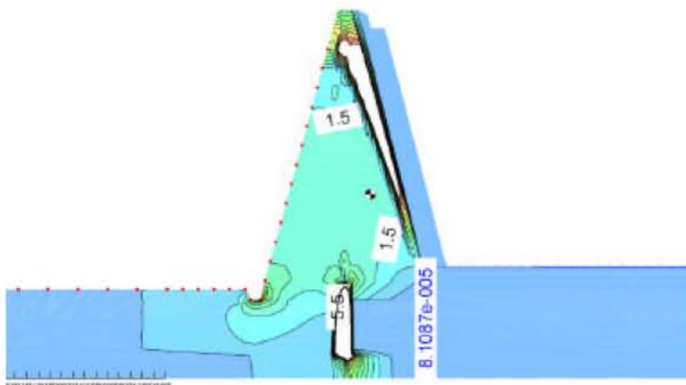
Fig. 8: Model with up and down streams with drain and filter
