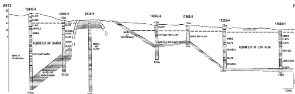
Fig. 2: Longitudinal section through the aquifer of El Khairat (Menaoui et al. , 1996).
