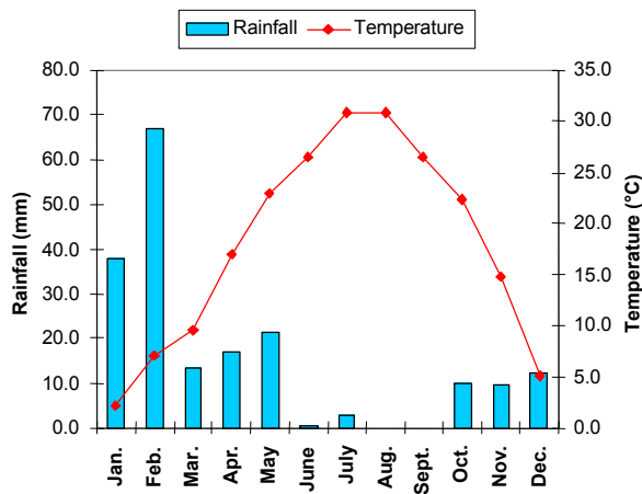
Fig. 5: Mean monthly rainfall and temperature data of the research site during the study years 2013 and 2014
