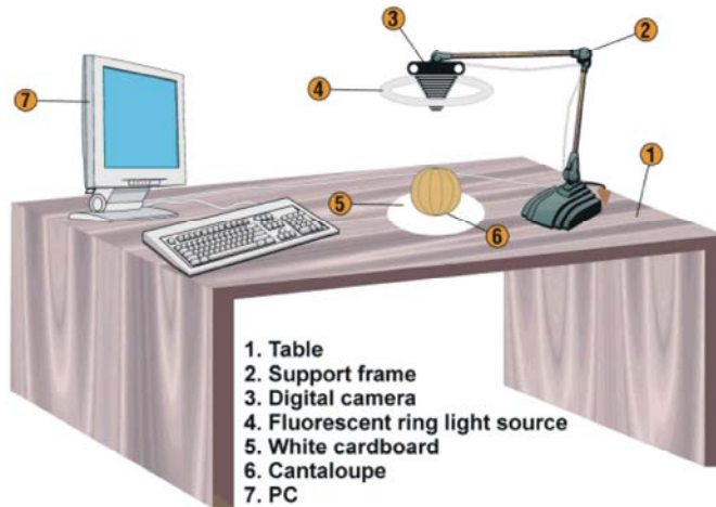
Fig. 1: Image acquisition system
